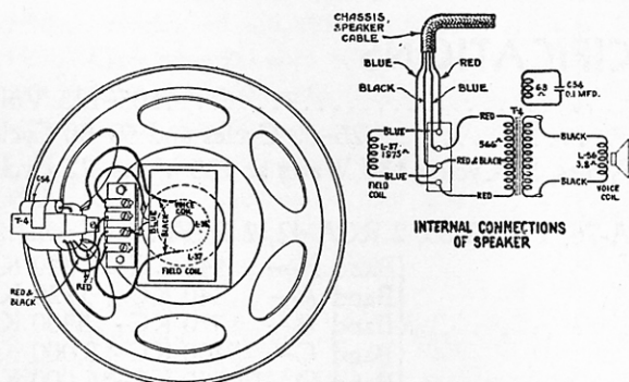
Figure 1—Loudspeaker Wiring—Without Plug
