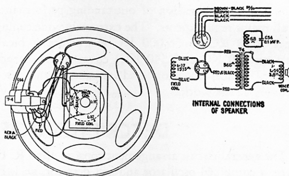
Figure 2—Loudspeaker Wiring for Plug-In Type
